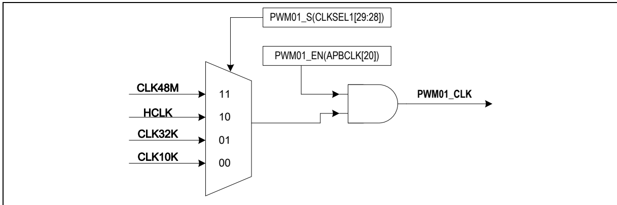
Figure 5-24 PWM Generator Clock Source Control
